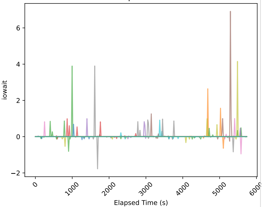
Traces of iowait for each cpu with utilization reaches 100%
