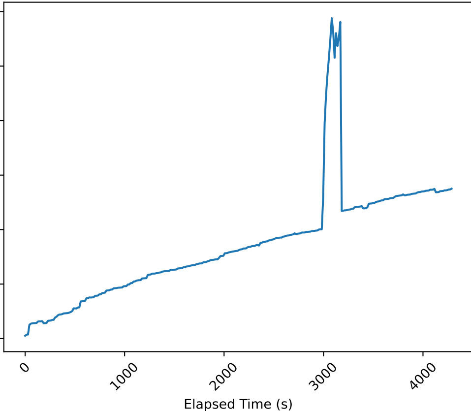
Traces of kbactive
