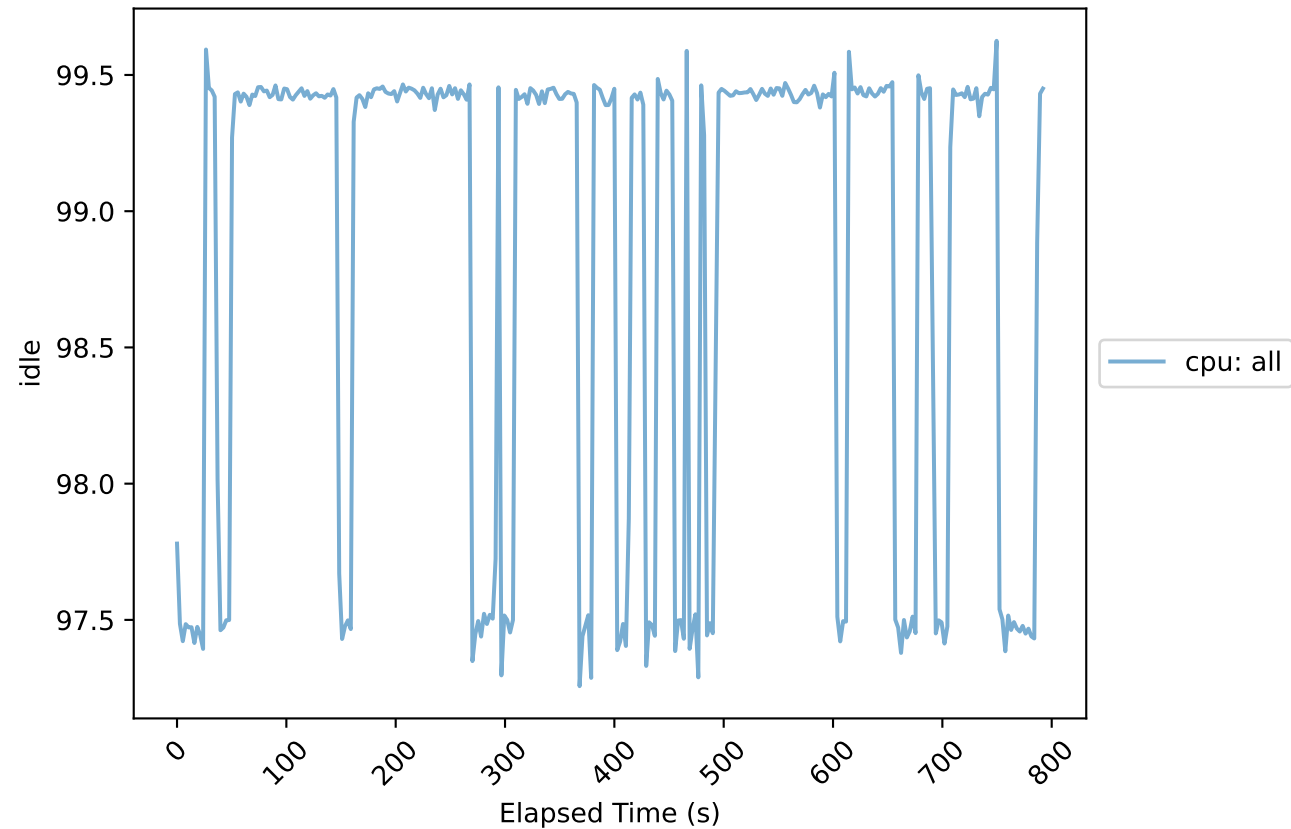
Traces of idle for each cpu
