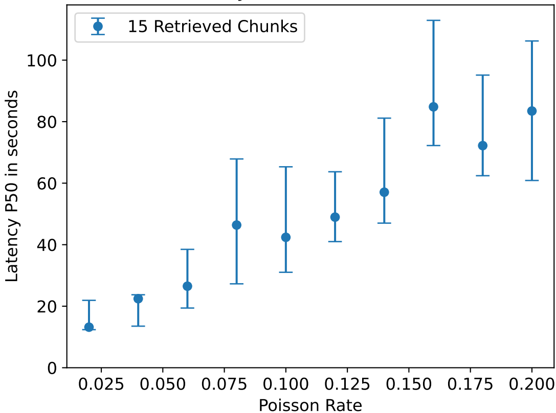
Latency P50 vs Poisson Rate
