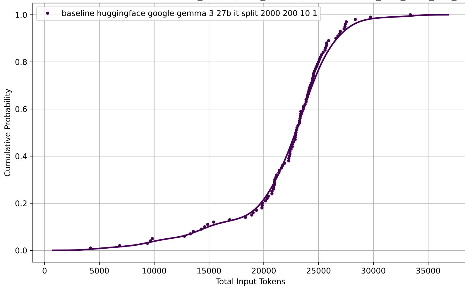
CDF of Total Input Tokens for baseline_huggingface_google-gemma-3-27b-it_split_2000_200_10_1
