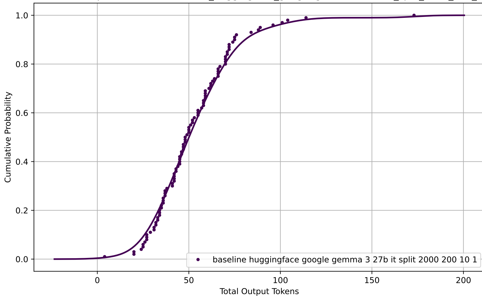
CDF of Total Output Tokens for baseline_huggingface_google-gemma-3-27b-it_split_2000_200_10_1
