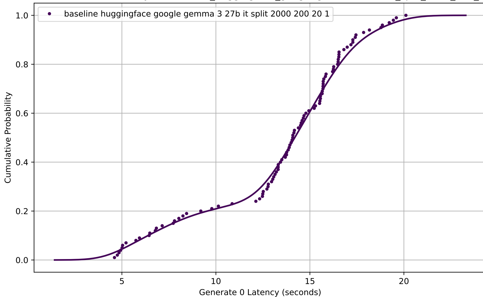
CDF of Generate 0 Latency for baseline_huggingface_google-gemma-3-27b-it_split_2000_200_20_1
