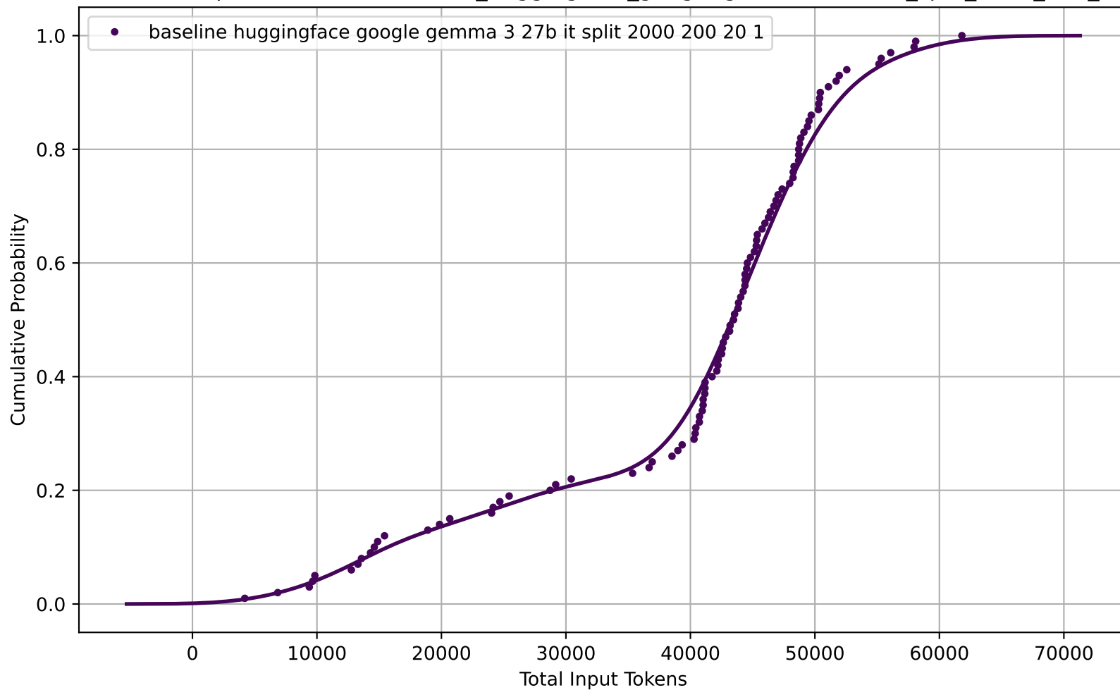
CDF of Total Input Tokens for baseline_huggingface_google-gemma-3-27b-it_split_2000_200_20_1
