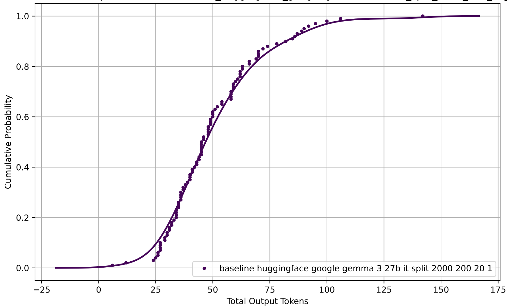
CDF of Total Output Tokens for baseline_huggingface_google-gemma-3-27b-it_split_2000_200_20_1
