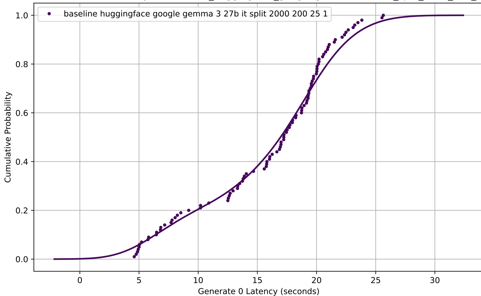
CDF of Generate 0 Latency for baseline_huggingface_google-gemma-3-27b-it_split_2000_200_25_1
