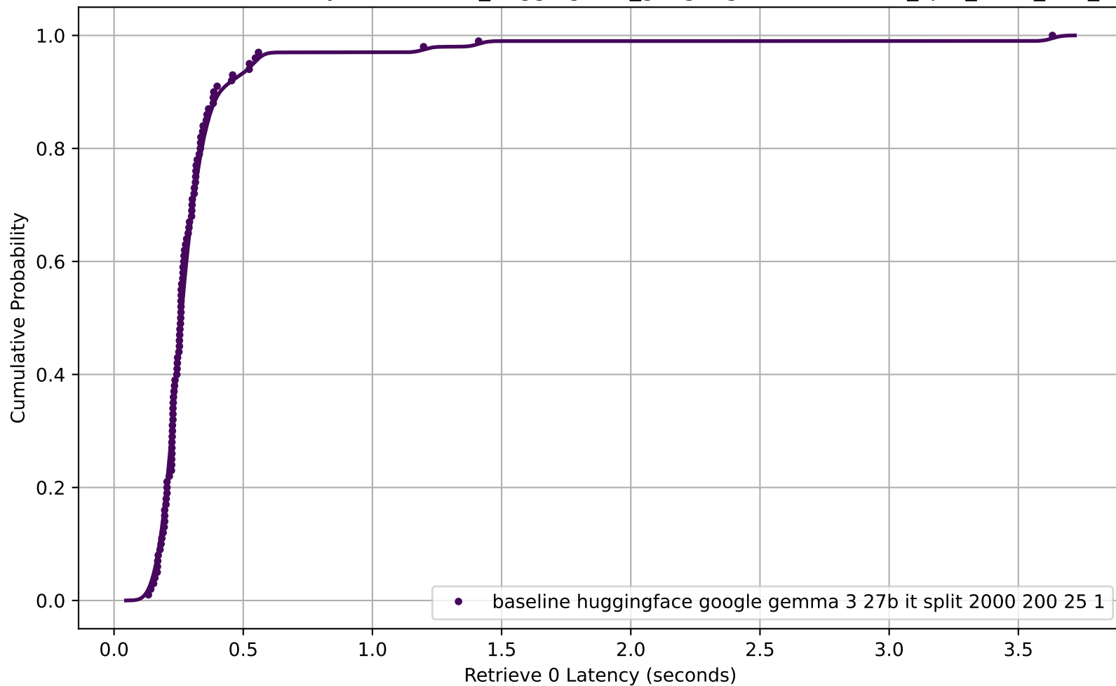
CDF of Retrieve 0 Latency for baseline_huggingface_google-gemma-3-27b-it_split_2000_200_25_1
