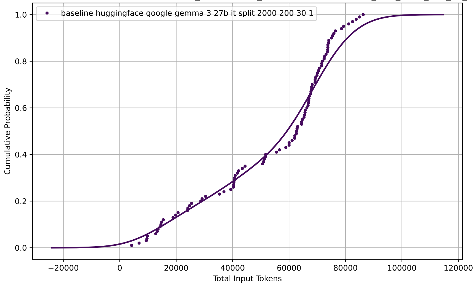
CDF of Total Input Tokens for baseline_huggingface_google-gemma-3-27b-it_split_2000_200_30_1
