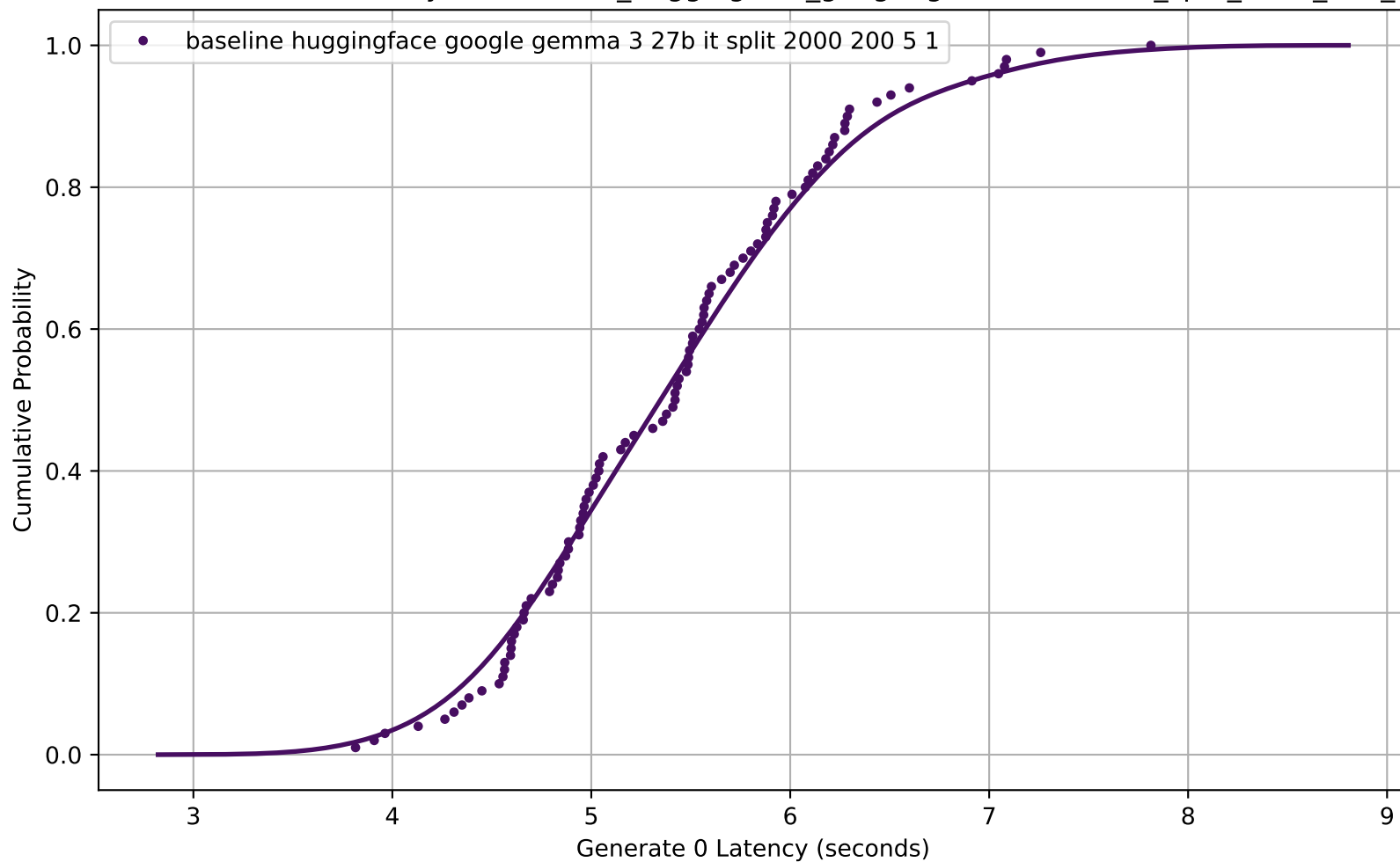
CDF of Generate 0 Latency for baseline_huggingface_google-gemma-3-27b-it_split_2000_200_5_1
