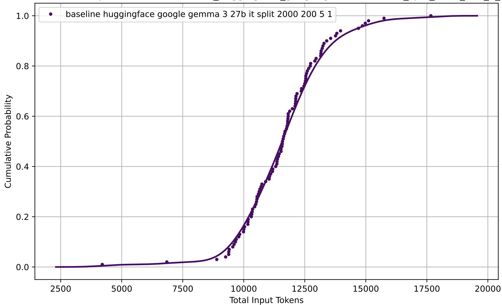
CDF of Total Input Tokens for baseline_huggingface_google-gemma-3-27b-it_split_2000_200_5_1
