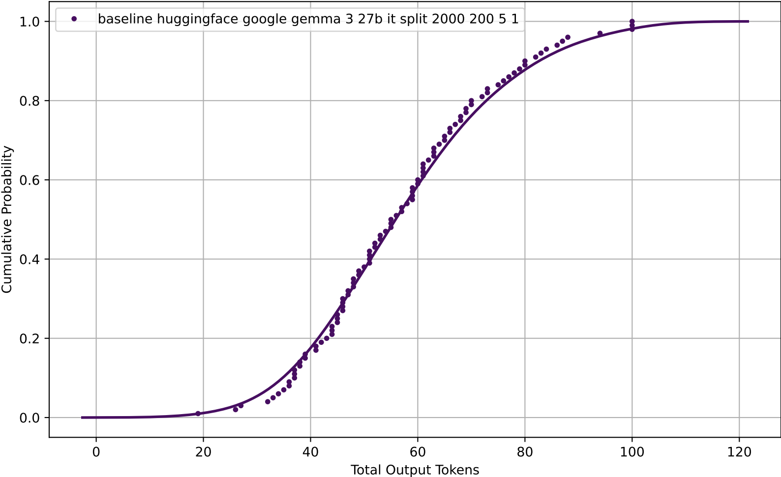
CDF of Total Output Tokens for baseline_huggingface_google-gemma-3-27b-it_split_2000_200_5_1
