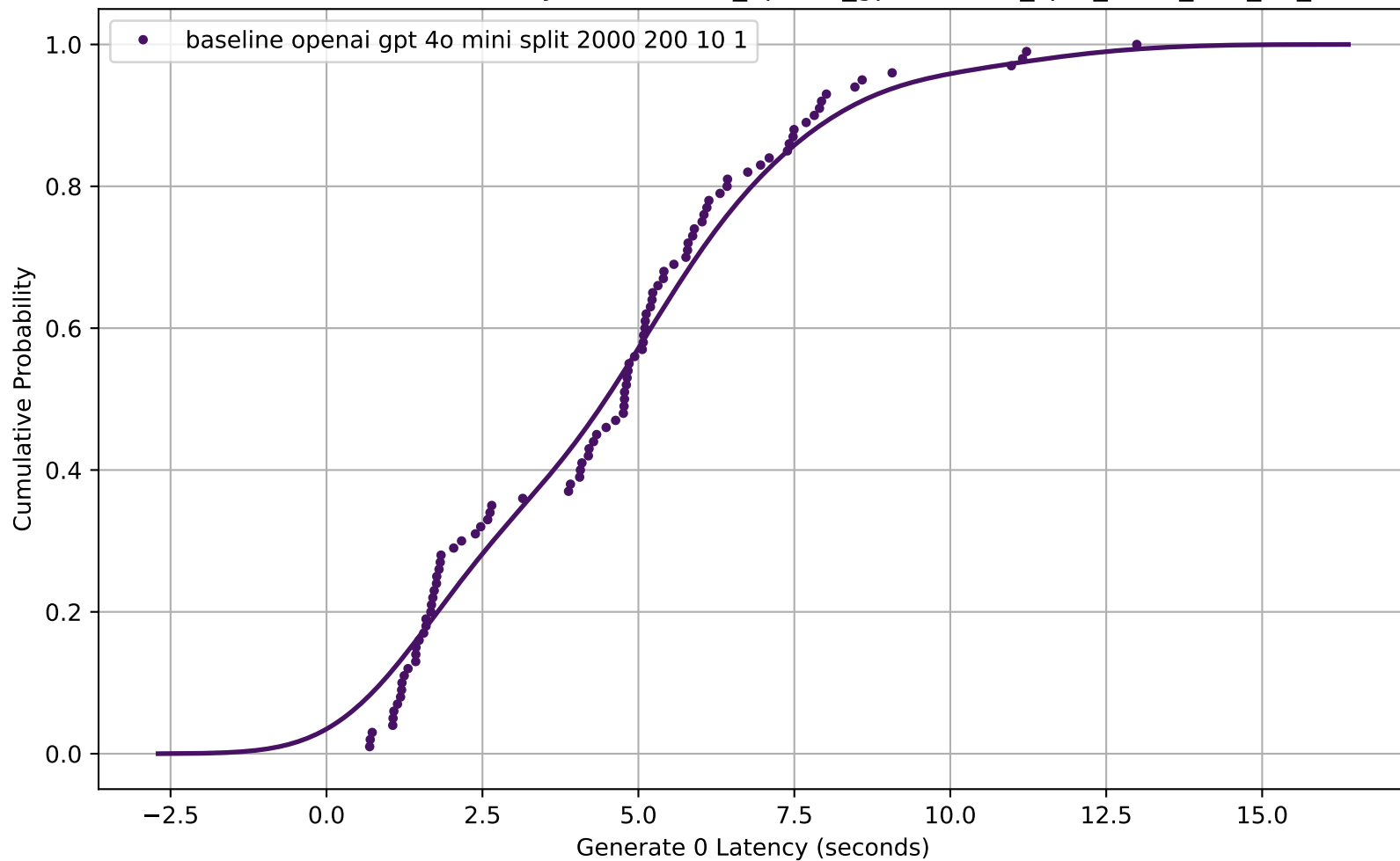
CDF of Generate 0 Latency for baseline_openai_gpt-4o-mini_split_2000_200_10_1
