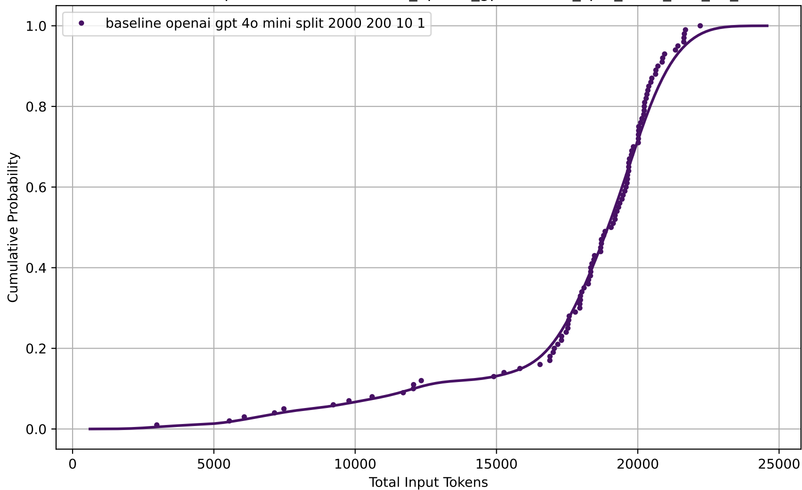
CDF of Total Input Tokens for baseline_openai_gpt-4o-mini_split_2000_200_10_1
