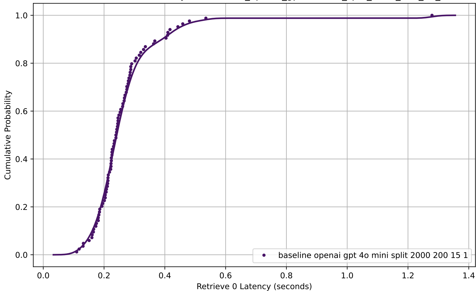
CDF of Retrieve 0 Latency for baseline_openai_gpt-4o-mini_split_2000_200_15_1
