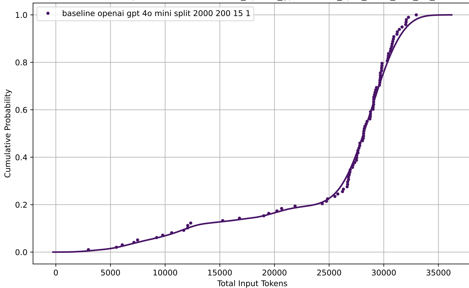
CDF of Total Input Tokens for baseline_openai_gpt-4o-mini_split_2000_200_15_1
