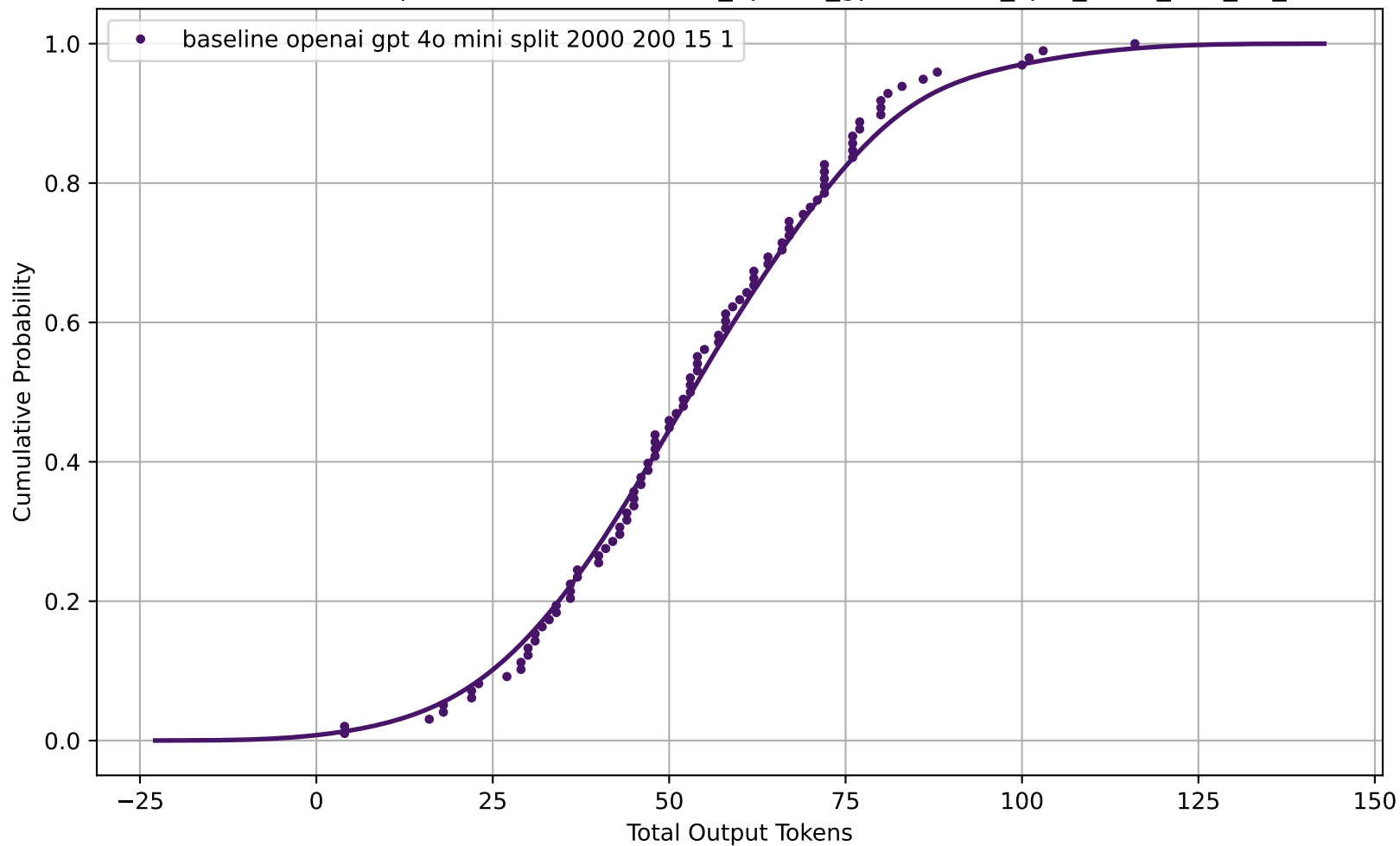
CDF of Total Output Tokens for baseline_openai_gpt-4o-mini_split_2000_200_15_1
