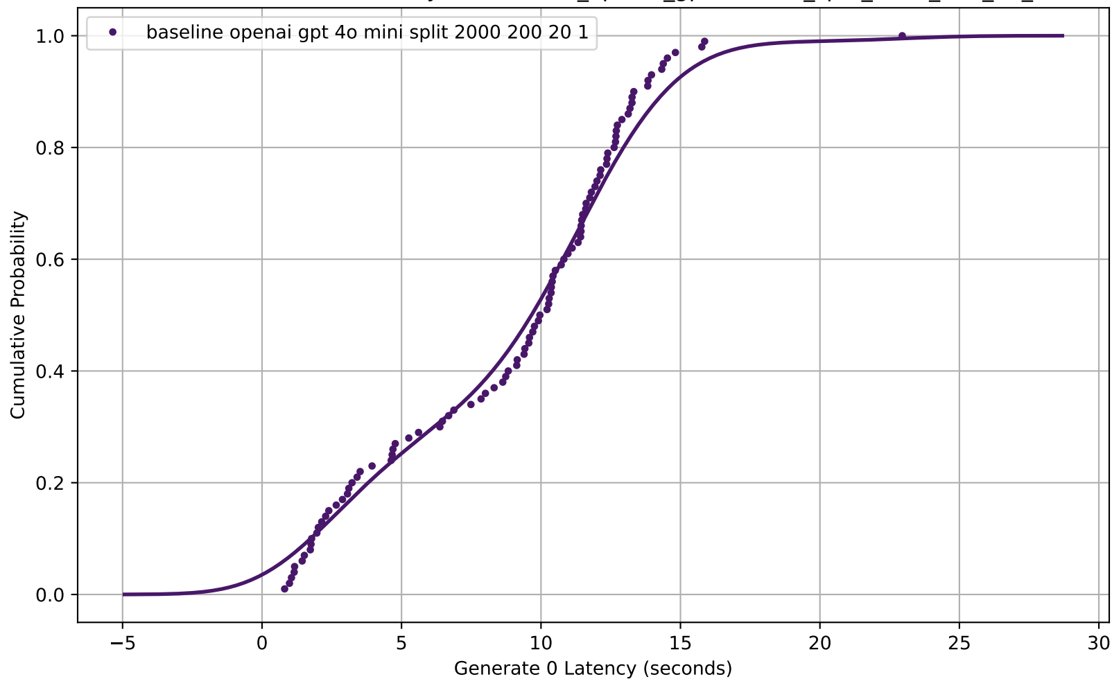
CDF of Generate 0 Latency for baseline_openai_gpt-4o-mini_split_2000_200_20_1
