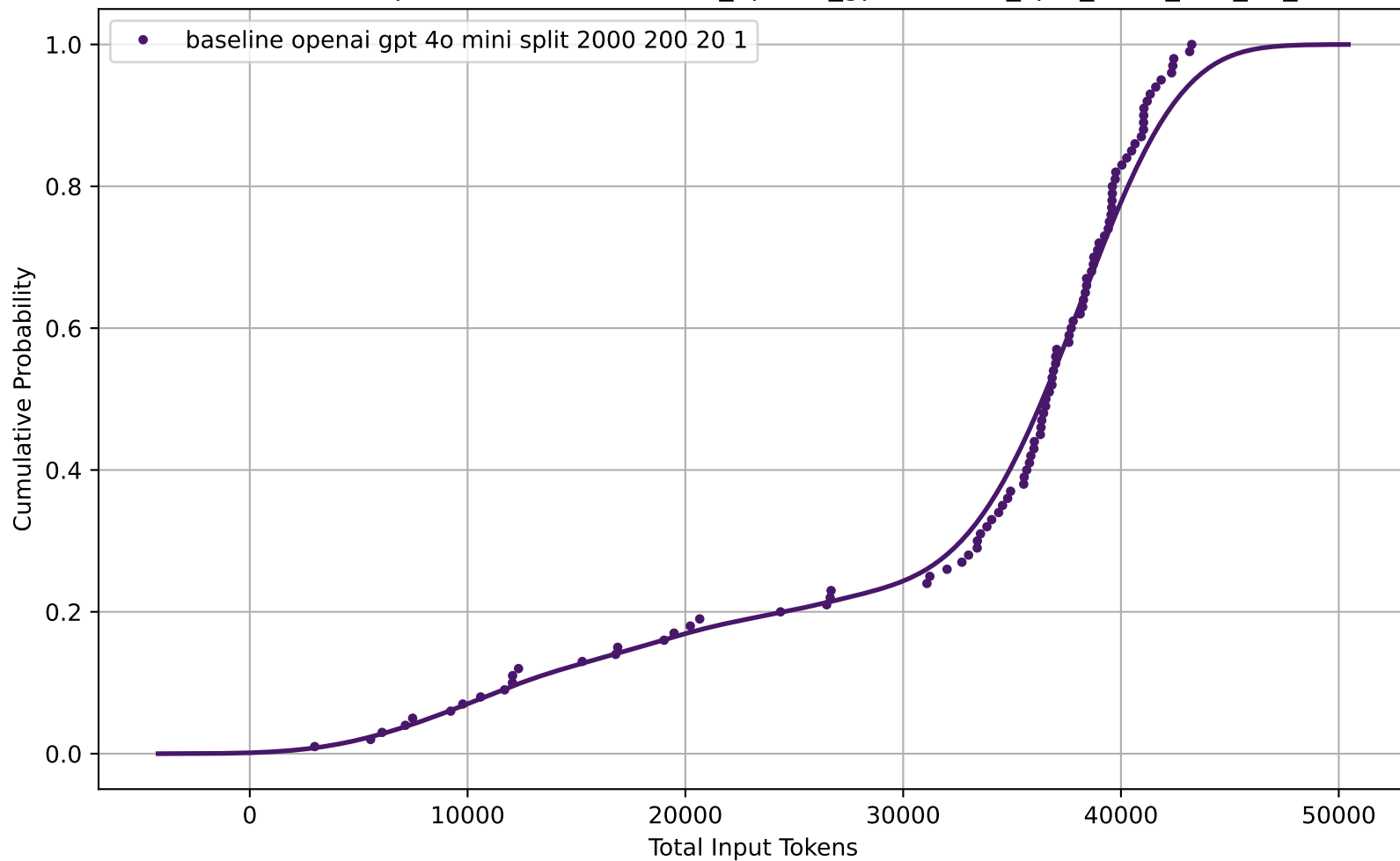
CDF of Total Input Tokens for baseline_openai_gpt-4o-mini_split_2000_200_20_1
