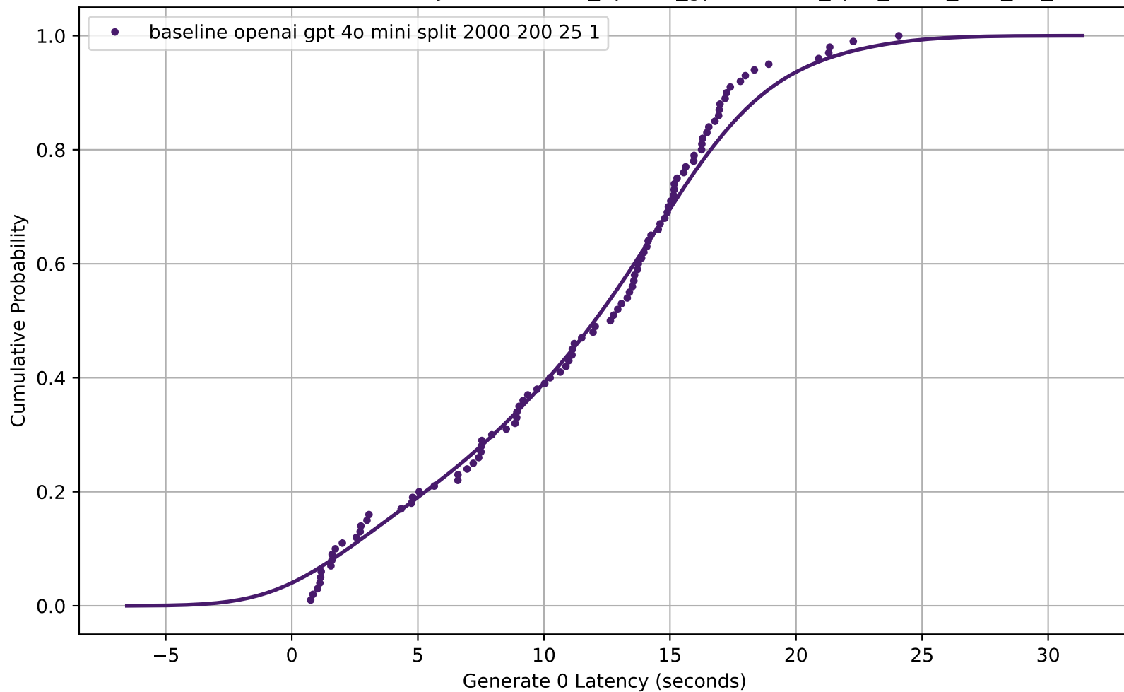
CDF of Generate 0 Latency for baseline_openai_gpt-4o-mini_split_2000_200_25_1
