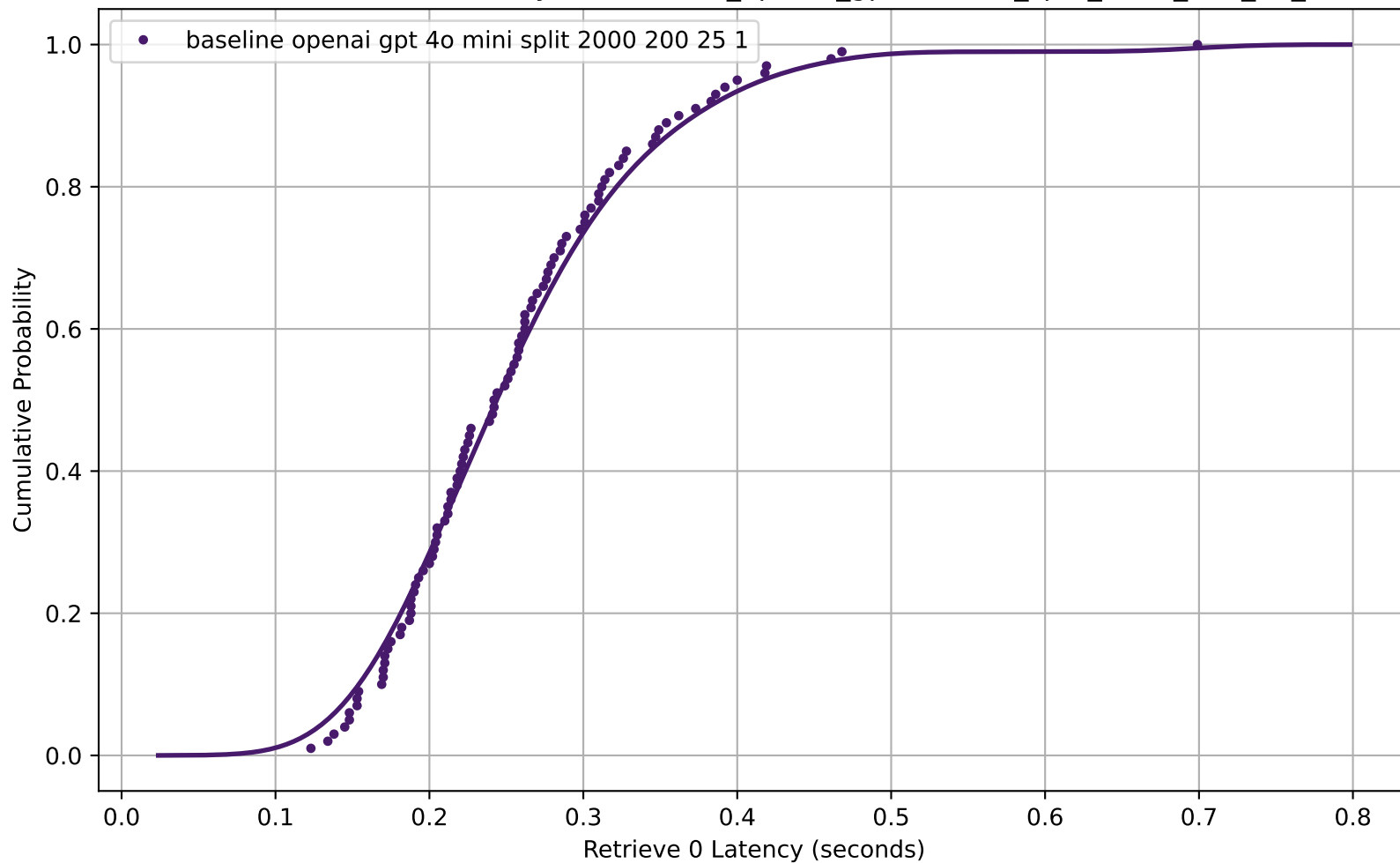
CDF of Retrieve 0 Latency for baseline_openai_gpt-4o-mini_split_2000_200_25_1
