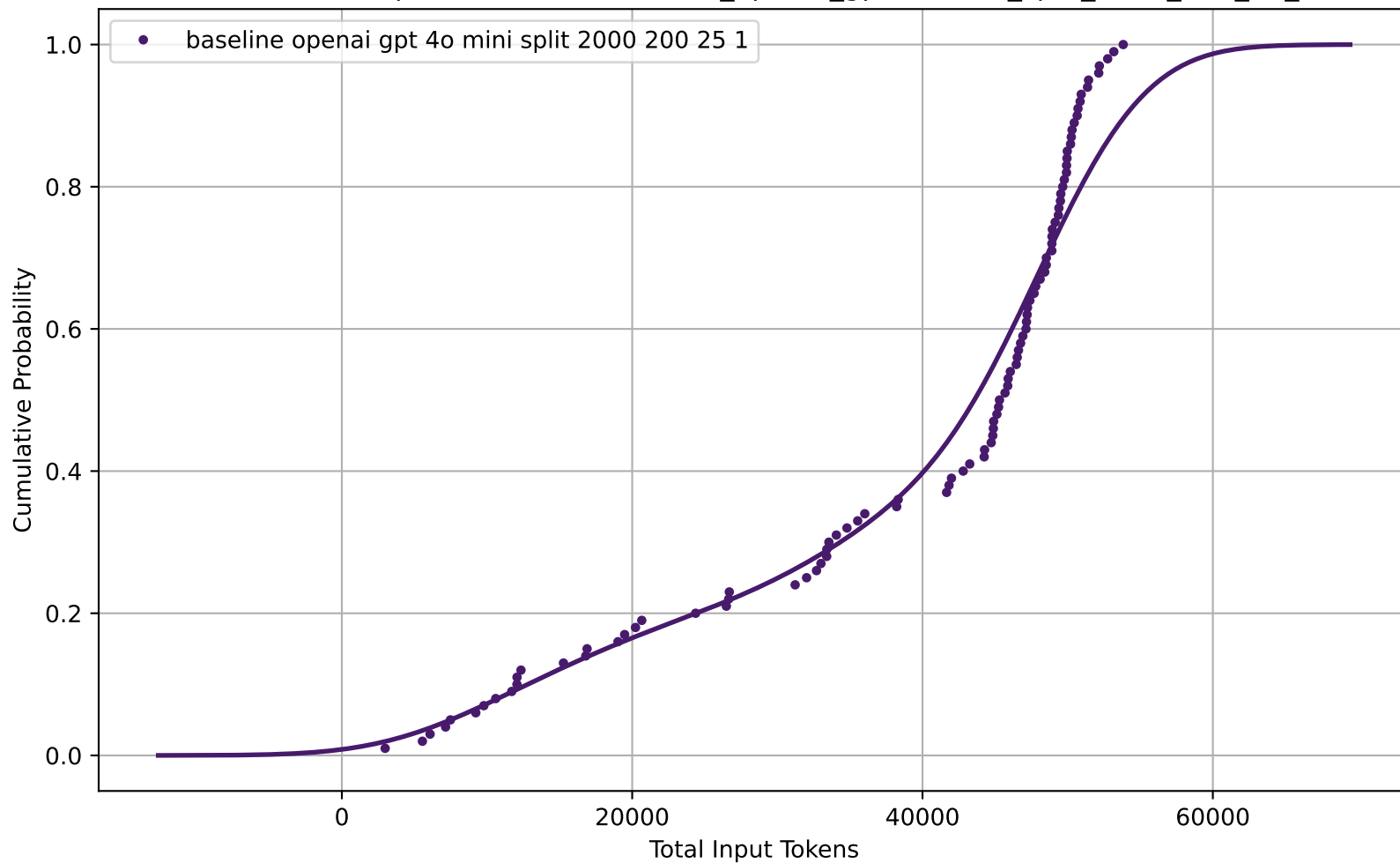
CDF of Total Input Tokens for baseline_openai_gpt-4o-mini_split_2000_200_25_1
