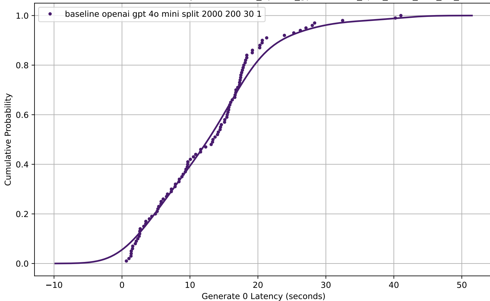
CDF of Generate 0 Latency for baseline_openai_gpt-4o-mini_split_2000_200_30_1
