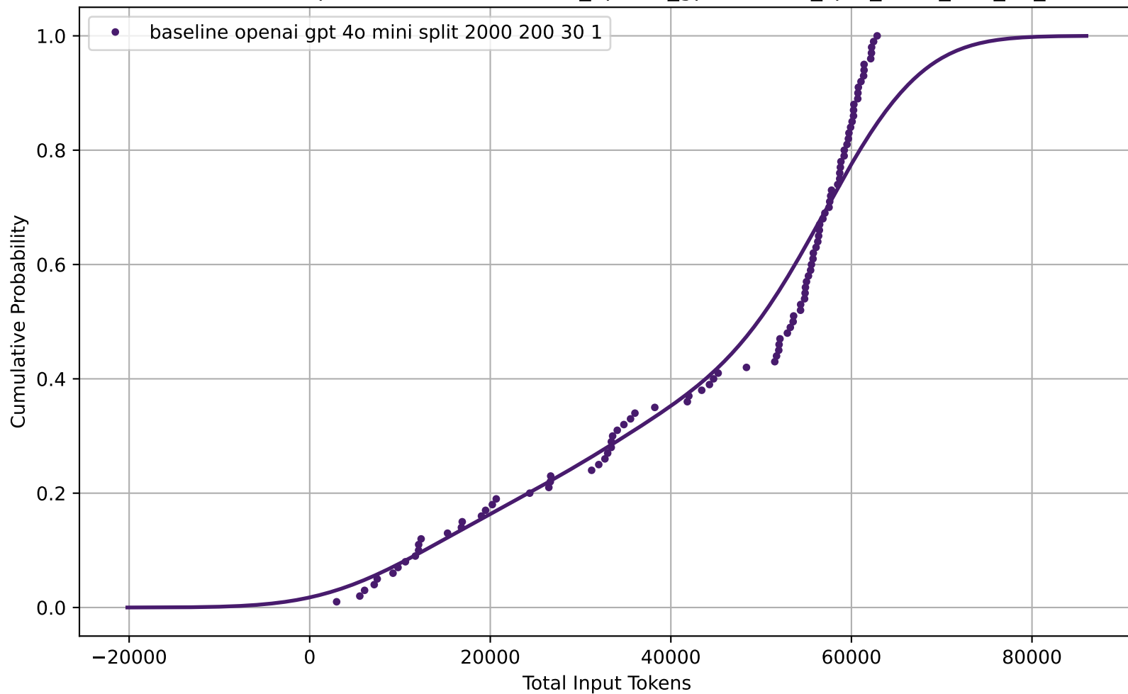
CDF of Total Input Tokens for baseline_openai_gpt-4o-mini_split_2000_200_30_1
