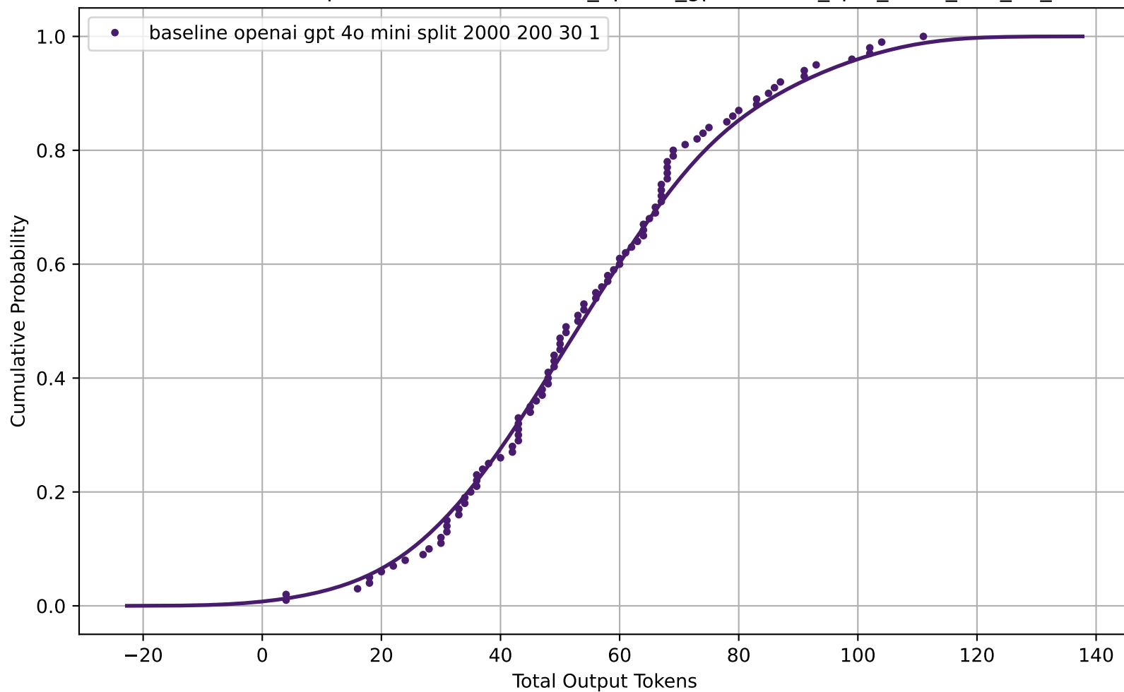
CDF of Total Output Tokens for baseline_openai_gpt-4o-mini_split_2000_200_30_1
