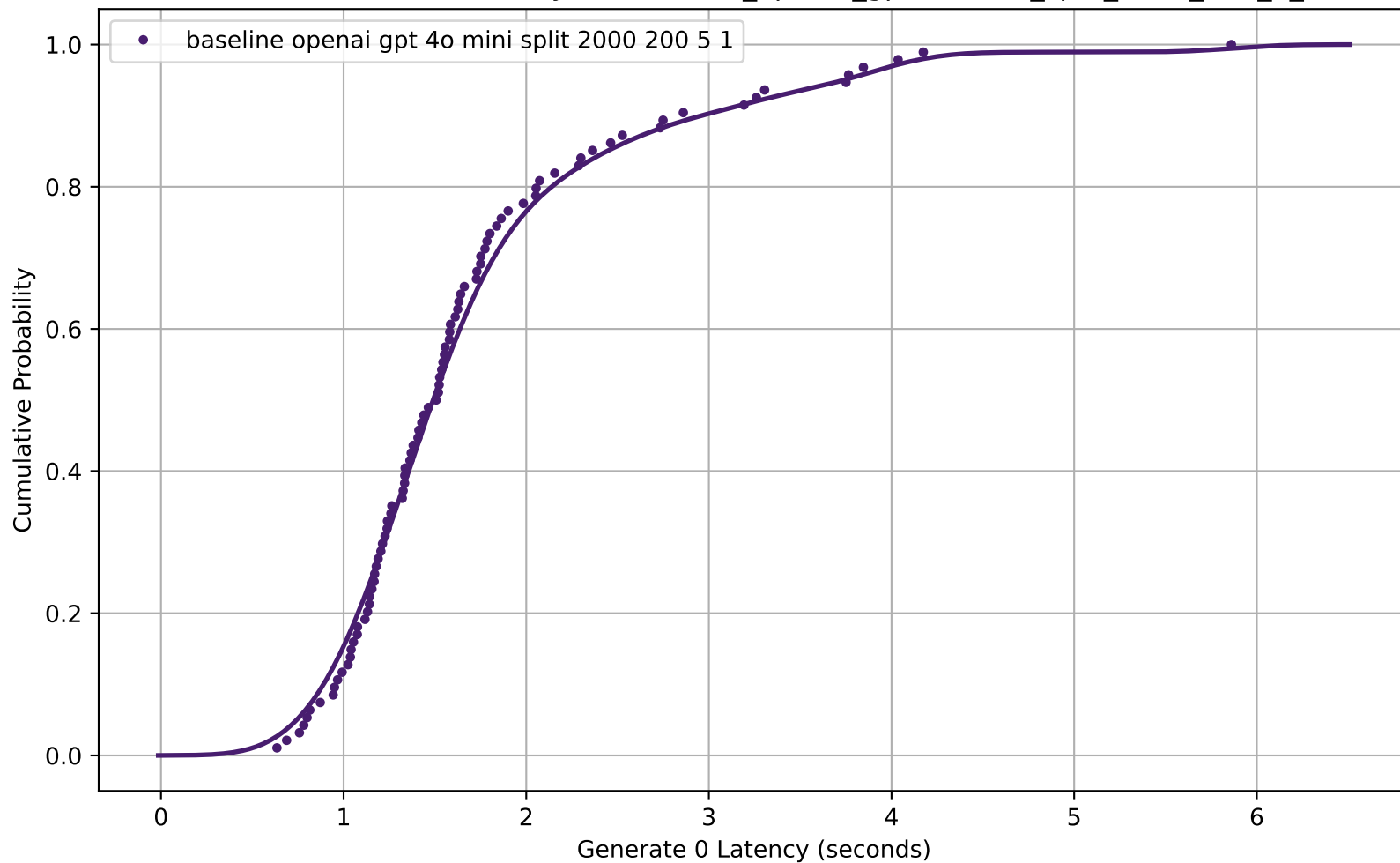
CDF of Generate 0 Latency for baseline_openai_gpt-4o-mini_split_2000_200_5_1
