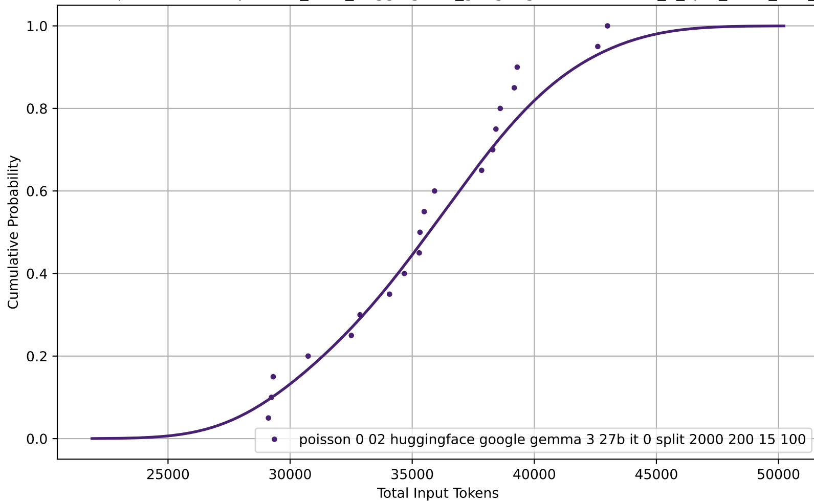
CDF of Total Input Tokens for poisson_0-02_huggingface_google-gemma-3-27b-it_0_split_2000_200_15_100
