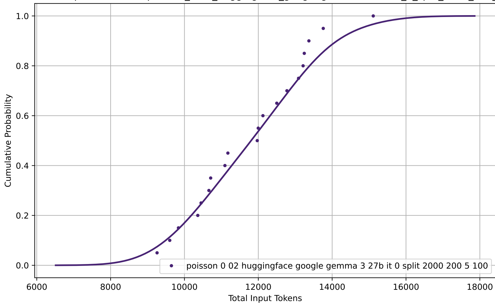
CDF of Total Input Tokens for poisson_0-02_huggingface_google-gemma-3-27b-it_0_split_2000_200_5_100
