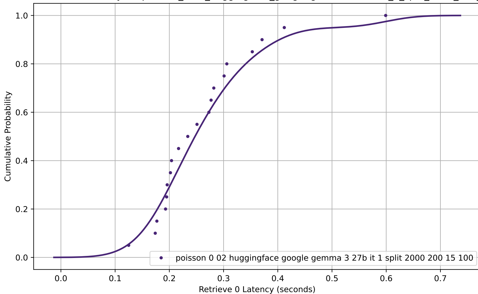
CDF of Retrieve 0 Latency for poisson_0-02_huggingface_google-gemma-3-27b-it_1_split_2000_200_15_100
