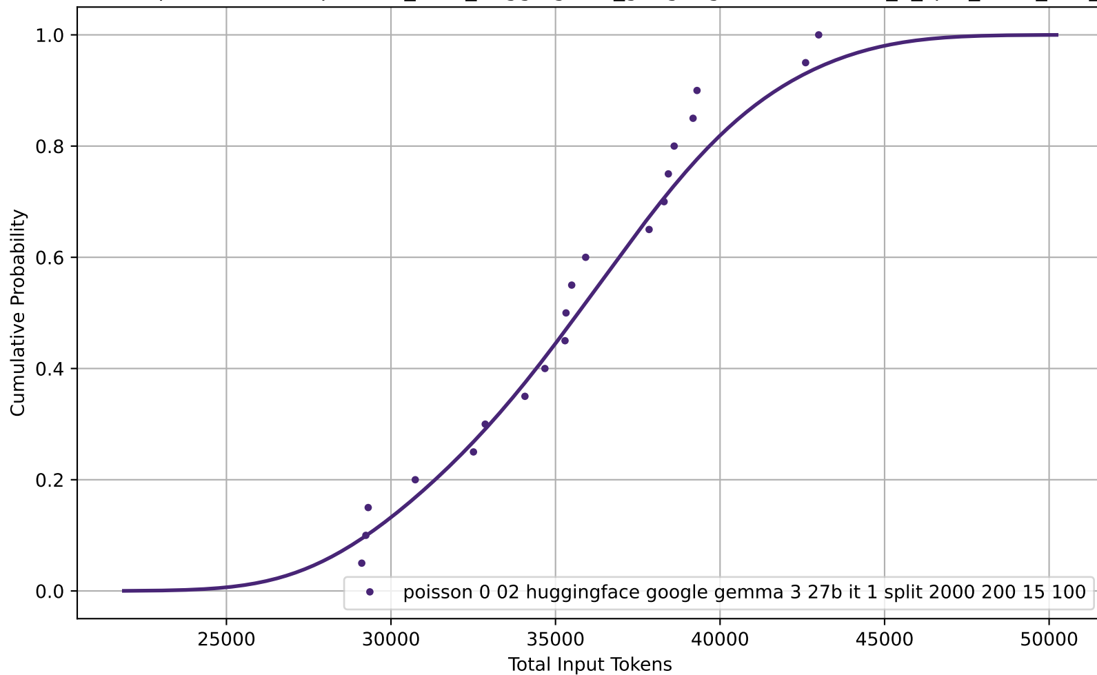
CDF of Total Input Tokens for poisson_0-02_huggingface_google-gemma-3-27b-it_1_split_2000_200_15_100
