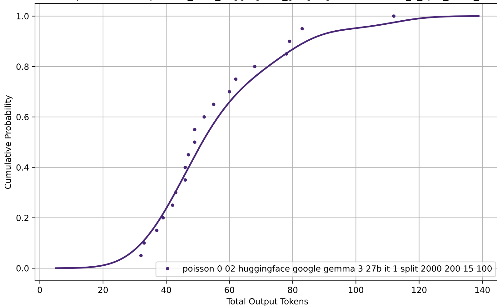
CDF of Total Output Tokens for poisson_0-02_huggingface_google-gemma-3-27b-it_1_split_2000_200_15_100
