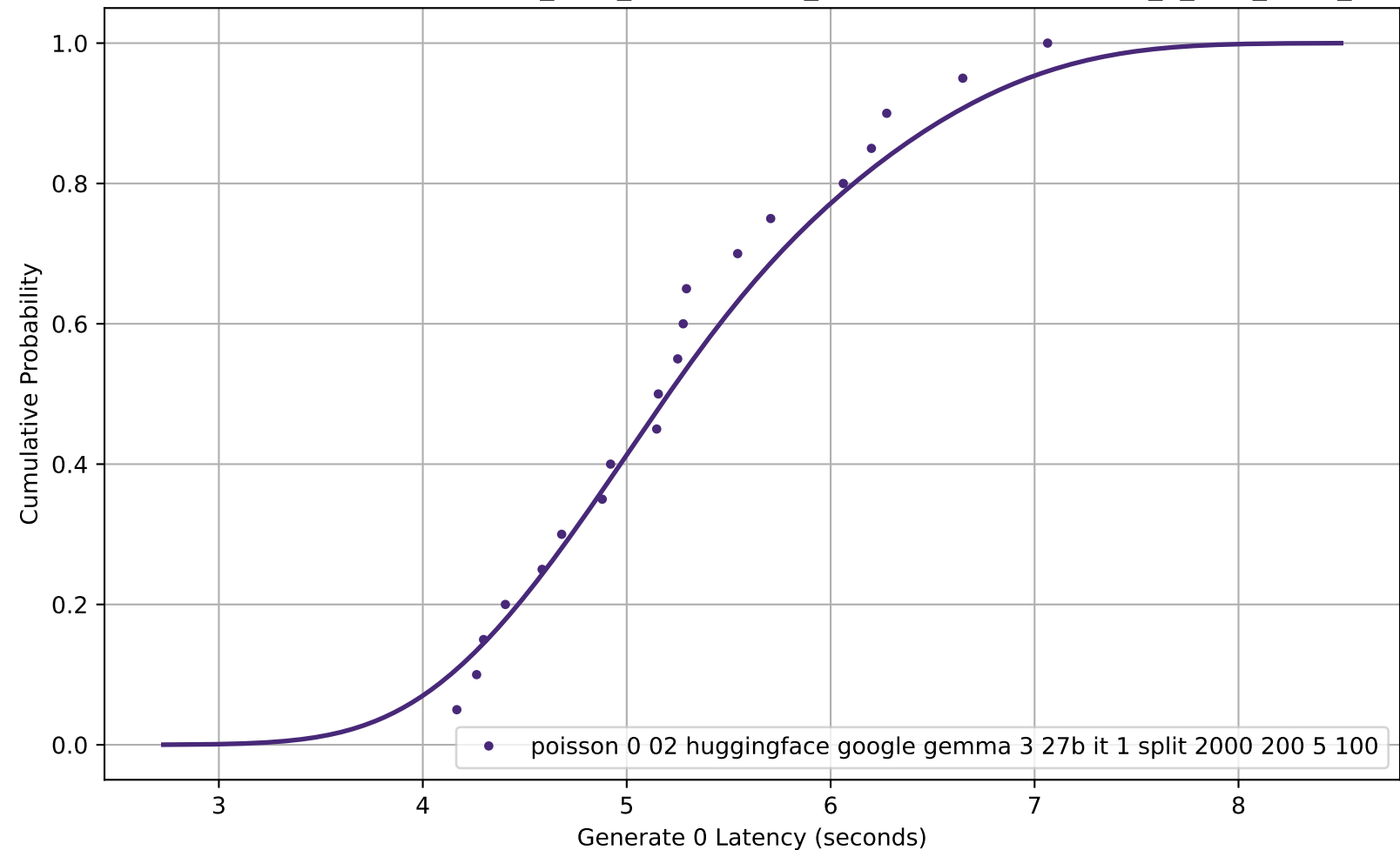
CDF of Generate 0 Latency for poisson_0-02_huggingface_google-gemma-3-27b-it_1_split_2000_200_5_100
