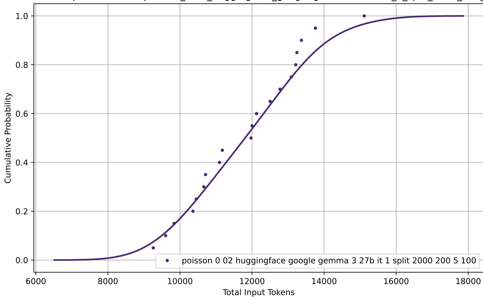
CDF of Total Input Tokens for poisson_0-02_huggingface_google-gemma-3-27b-it_1_split_2000_200_5_100
