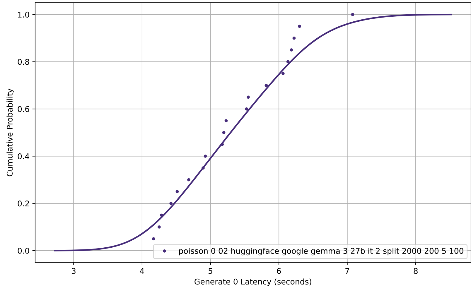
CDF of Generate 0 Latency for poisson_0-02_huggingface_google-gemma-3-27b-it_2_split_2000_200_5_100
