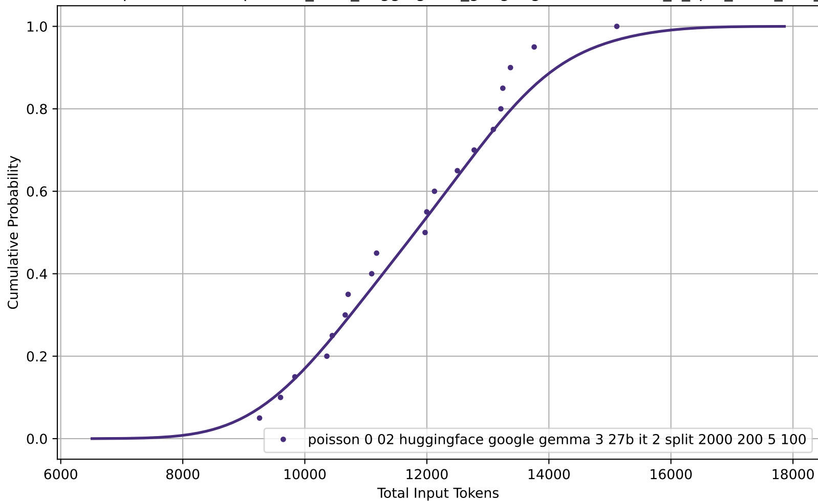
CDF of Total Input Tokens for poisson_0-02_huggingface_google-gemma-3-27b-it_2_split_2000_200_5_100
