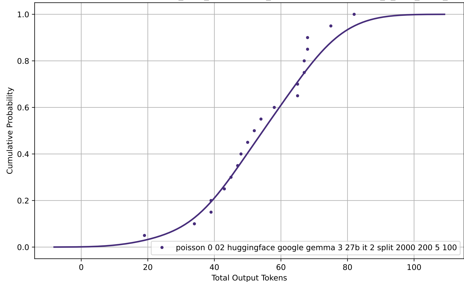
CDF of Total Output Tokens for poisson_0-02_huggingface_google-gemma-3-27b-it_2_split_2000_200_5_100
