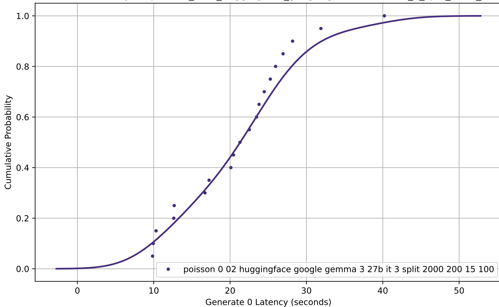
CDF of Generate 0 Latency for poisson_0-02_huggingface_google-gemma-3-27b-it_3_split_2000_200_15_100
