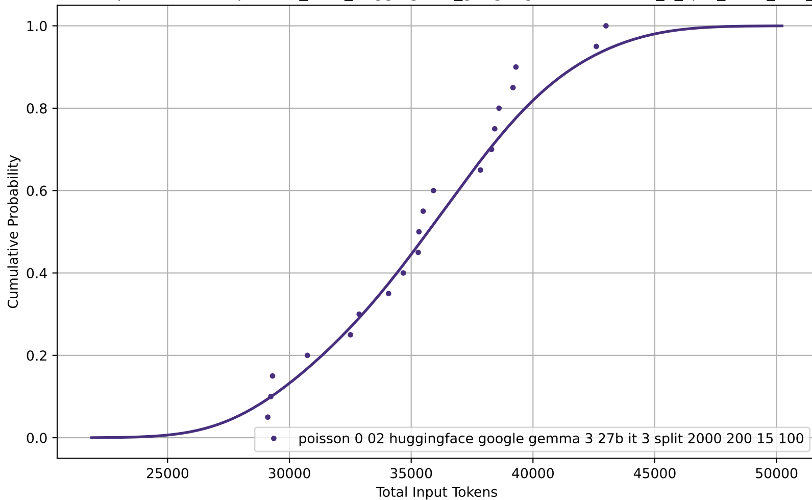
CDF of Total Input Tokens for poisson_0-02_huggingface_google-gemma-3-27b-it_3_split_2000_200_15_100
