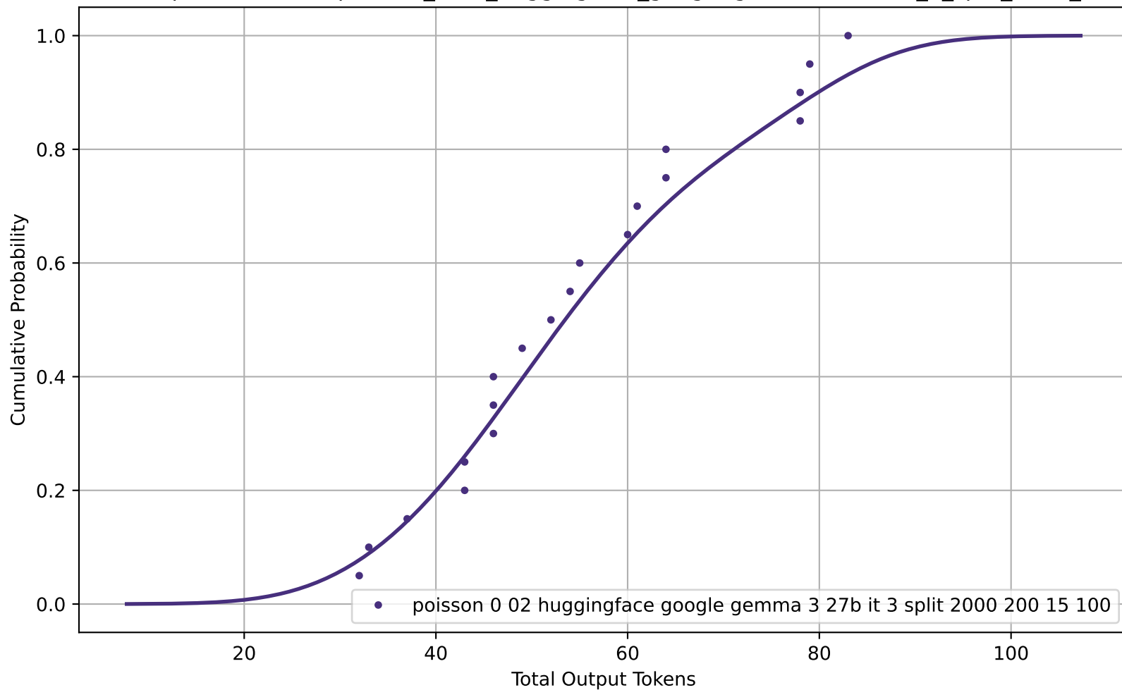
CDF of Total Output Tokens for poisson_0-02_huggingface_google-gemma-3-27b-it_3_split_2000_200_15_100
