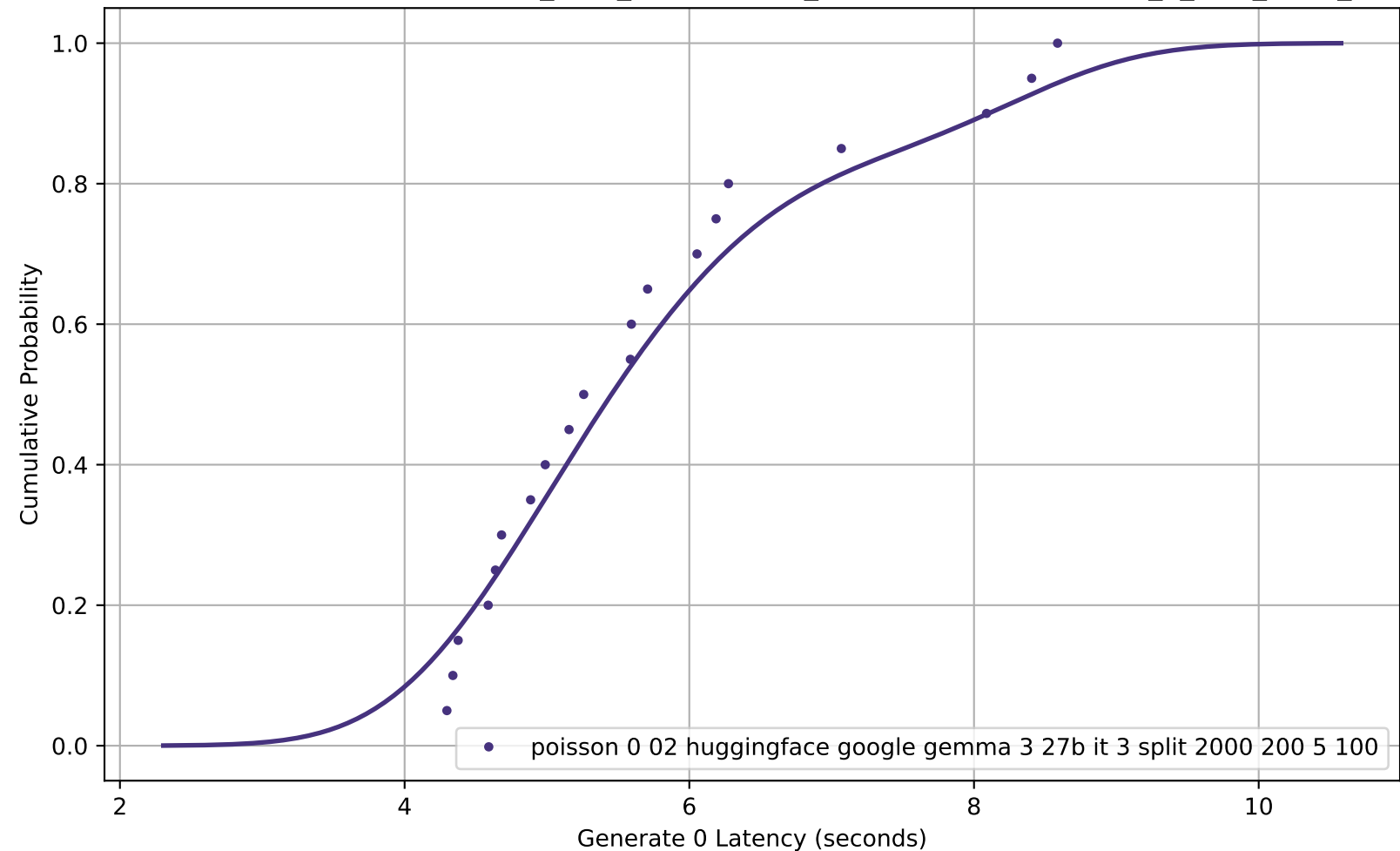
CDF of Generate 0 Latency for poisson_0-02_huggingface_google-gemma-3-27b-it_3_split_2000_200_5_100
