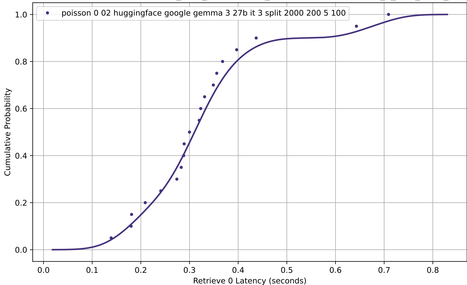
CDF of Retrieve 0 Latency for poisson_0-02_huggingface_google-gemma-3-27b-it_3_split_2000_200_5_100
