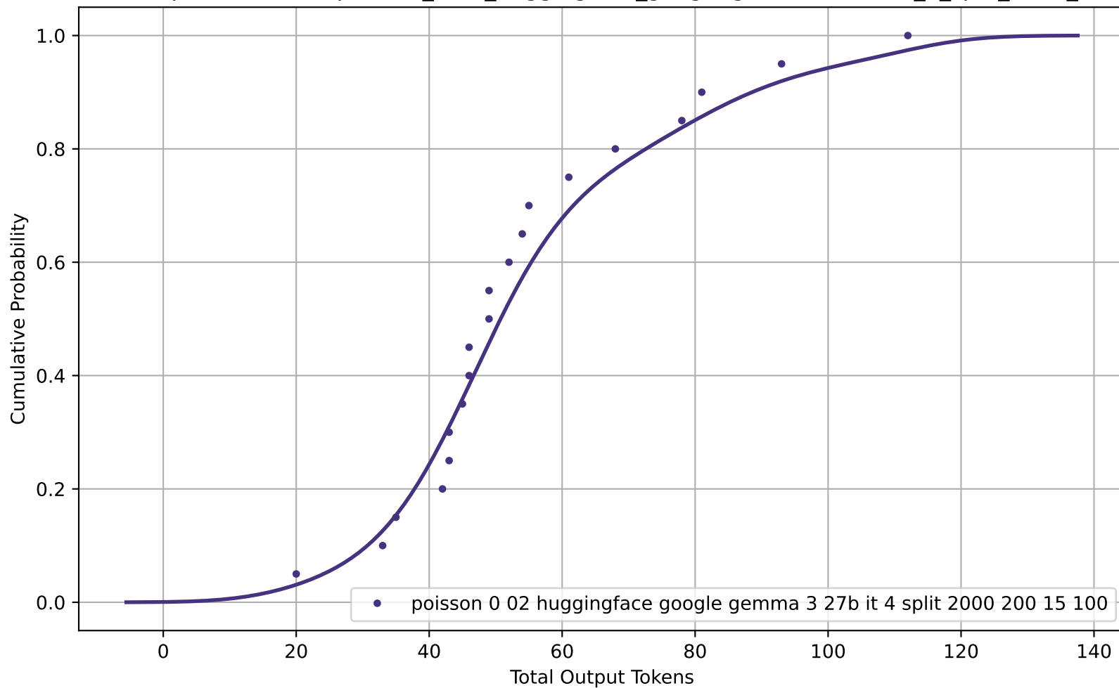
CDF of Total Output Tokens for poisson_0-02_huggingface_google-gemma-3-27b-it_4_split_2000_200_15_100
