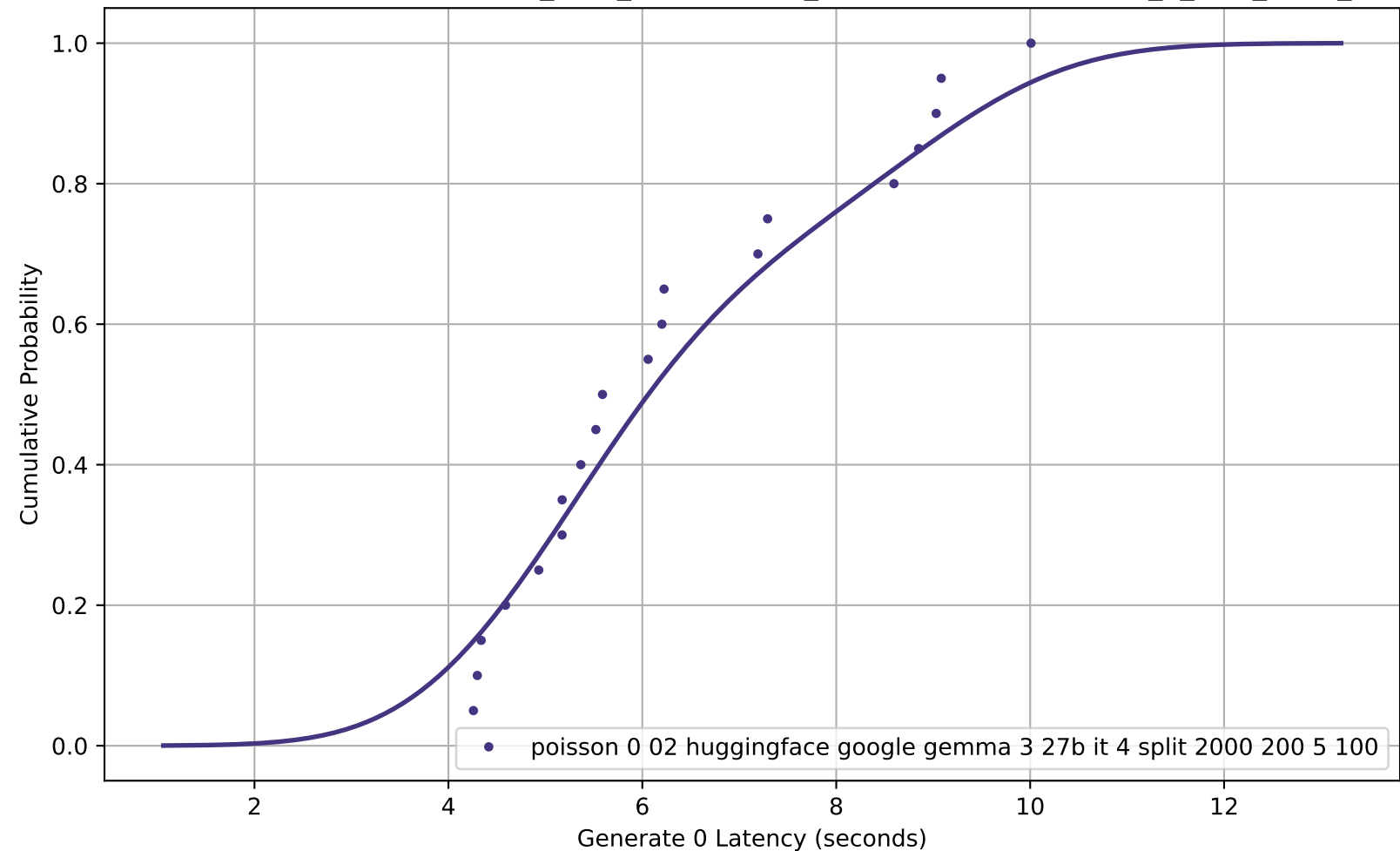
CDF of Generate 0 Latency for poisson_0-02_huggingface_google-gemma-3-27b-it_4_split_2000_200_5_100
