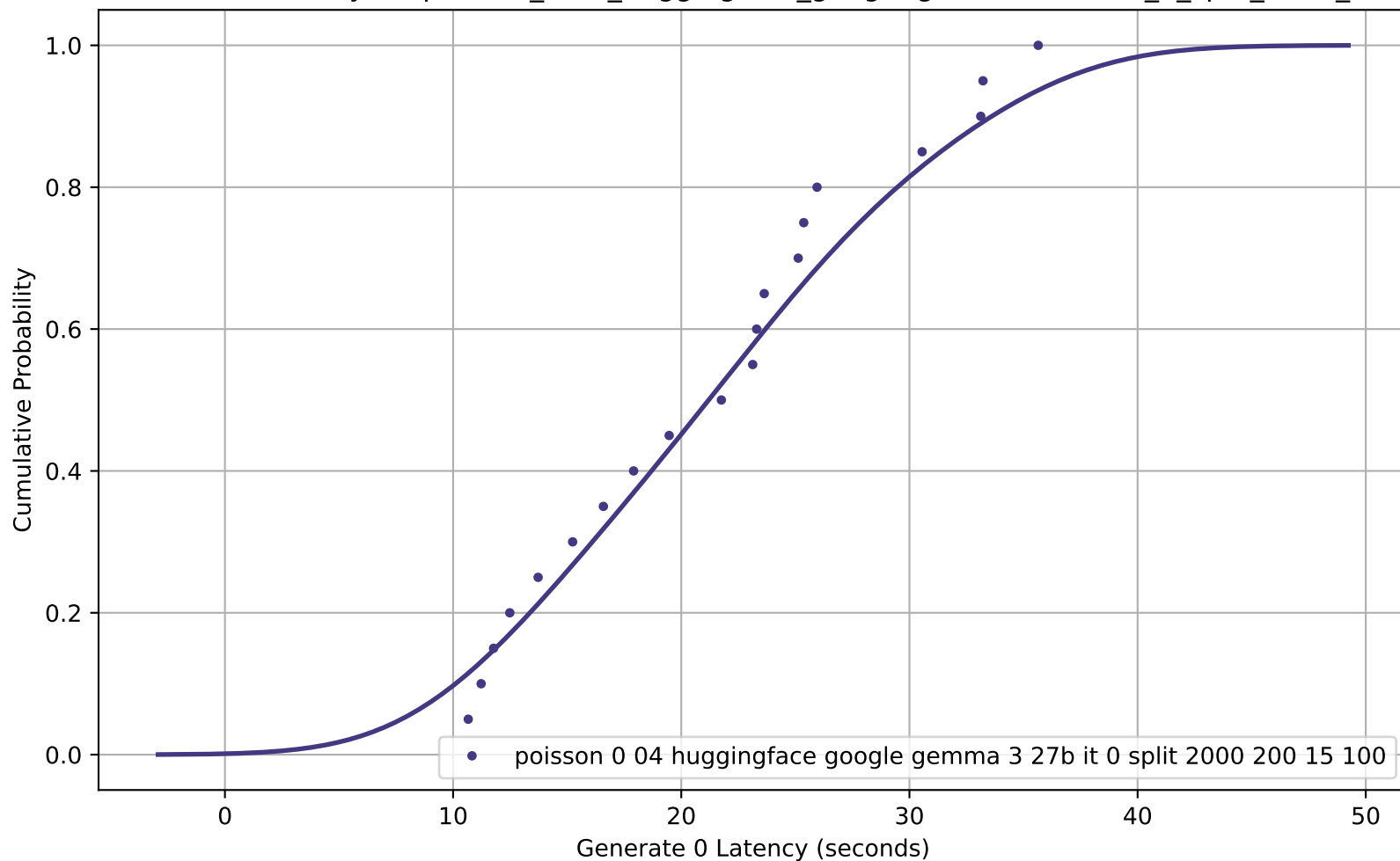
CDF of Generate 0 Latency for poisson_0-04_huggingface_google-gemma-3-27b-it_0_split_2000_200_15_100
