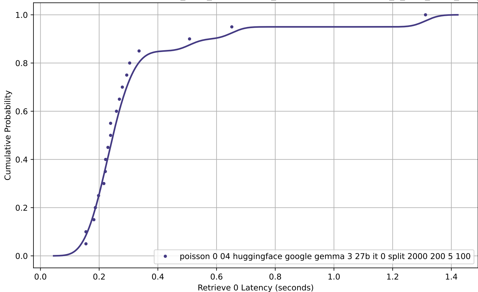
CDF of Retrieve 0 Latency for poisson_0-04_huggingface_google-gemma-3-27b-it_0_split_2000_200_5_100
