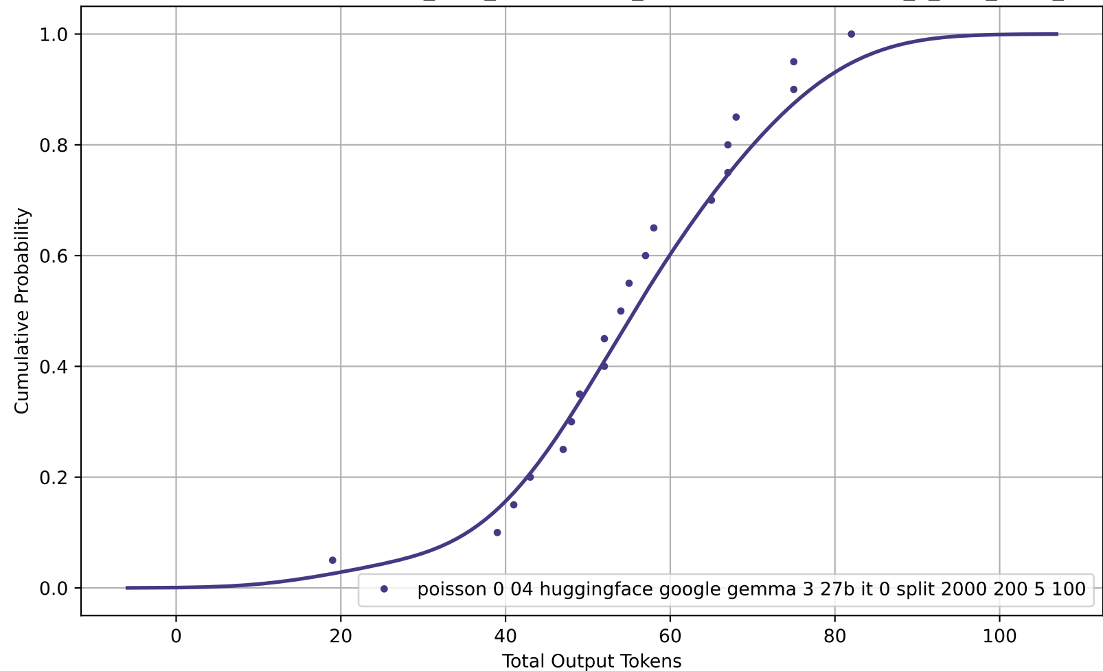
CDF of Total Output Tokens for poisson_0-04_huggingface_google-gemma-3-27b-it_0_split_2000_200_5_100
