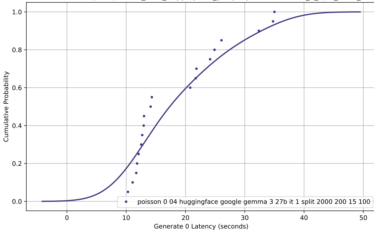
CDF of Generate 0 Latency for poisson_0-04_huggingface_google-gemma-3-27b-it_1_split_2000_200_15_100
